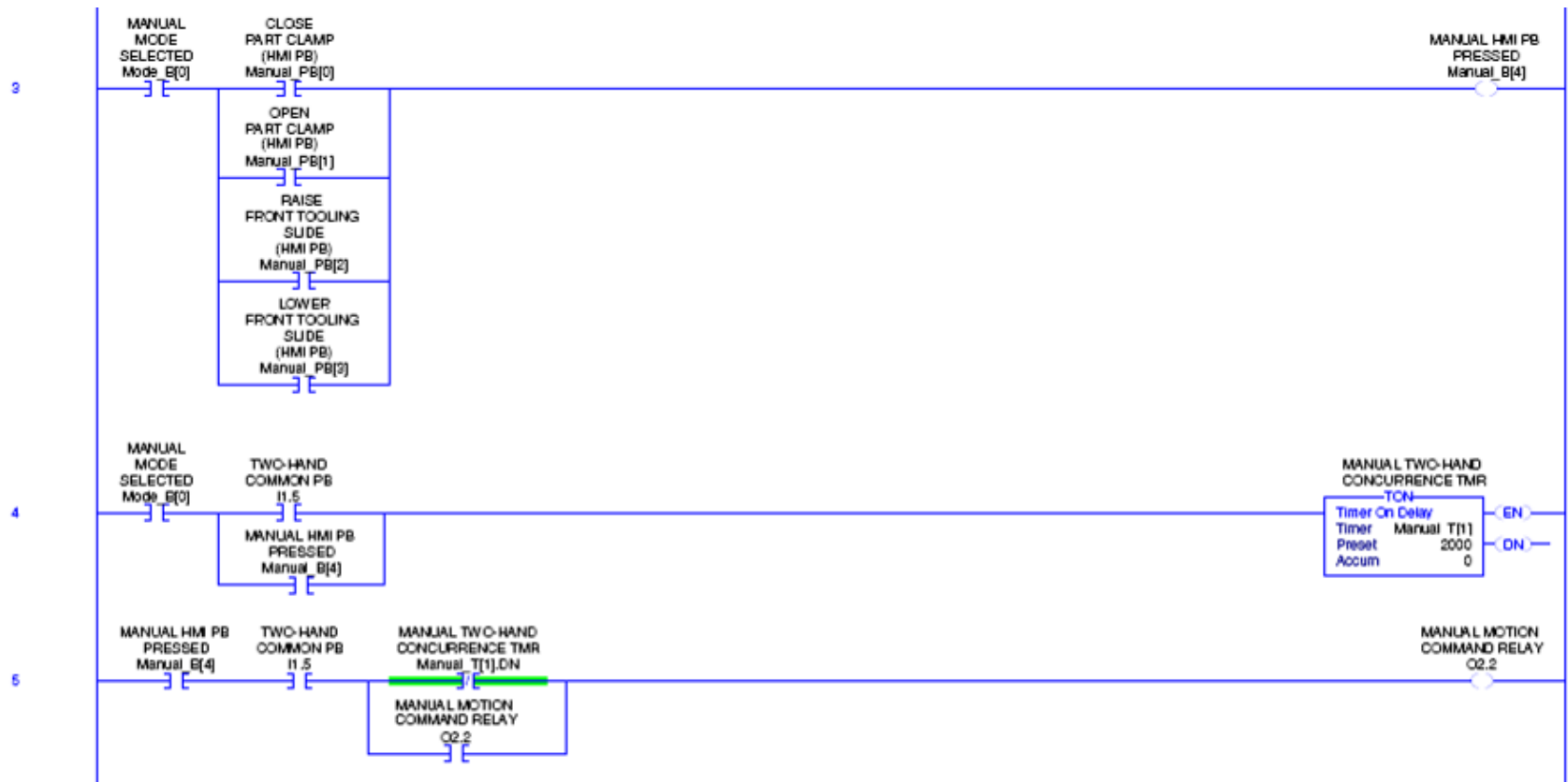
Figure 3.13.2.b –Category 2 Manual Motion Command Relay output logic
