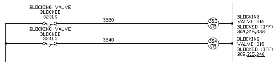
Figure 3.5.4.a - Feedback sensors controlling mechanically-linked relays
